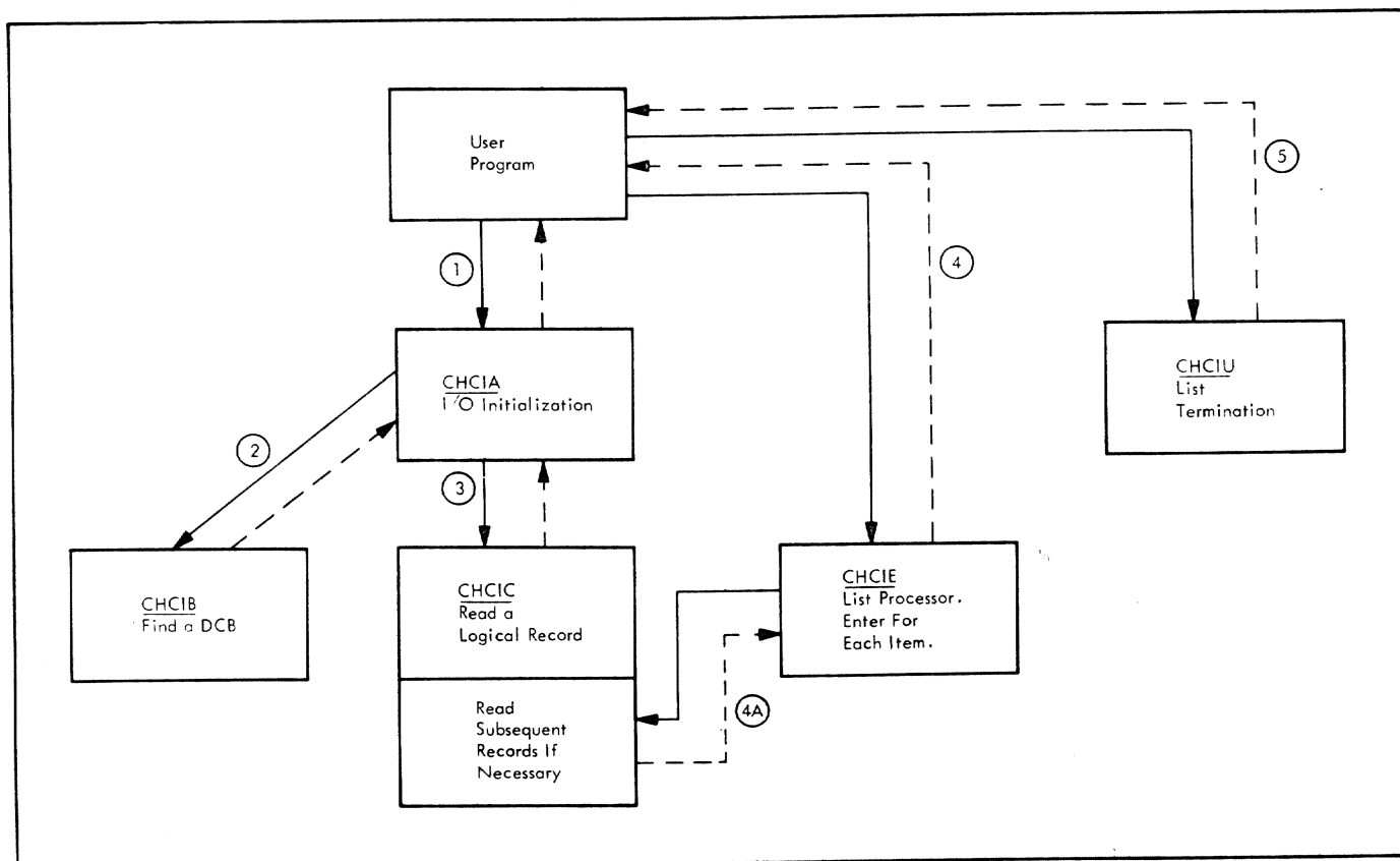
Figure 5. Unformatted READ with List
